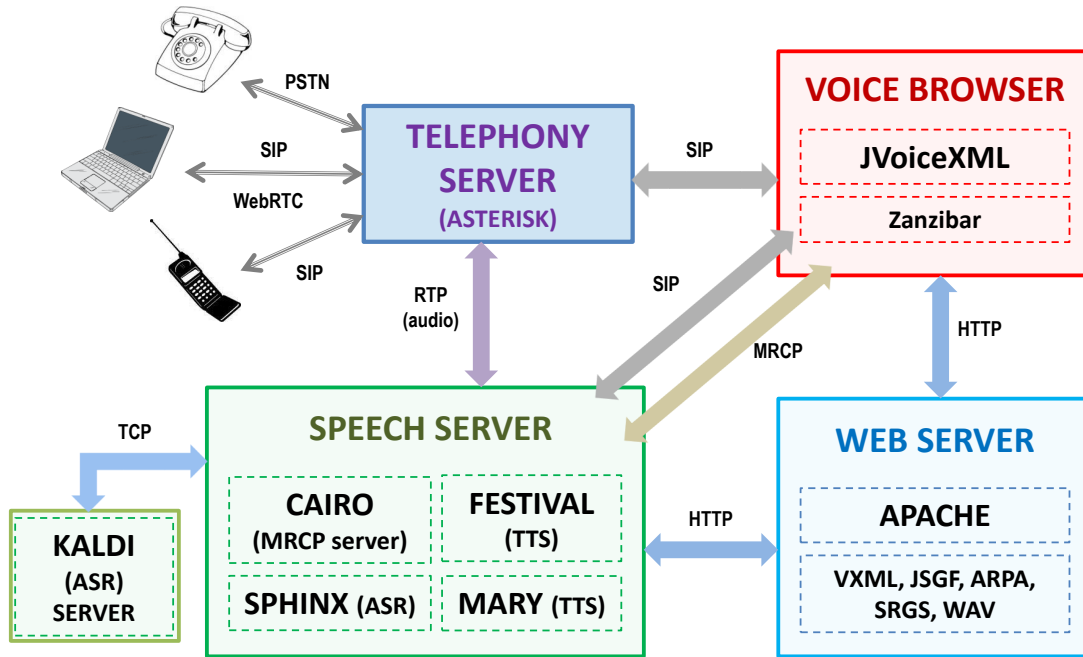
Figure 1: System architecture of the HALEF spoken dialog system.
